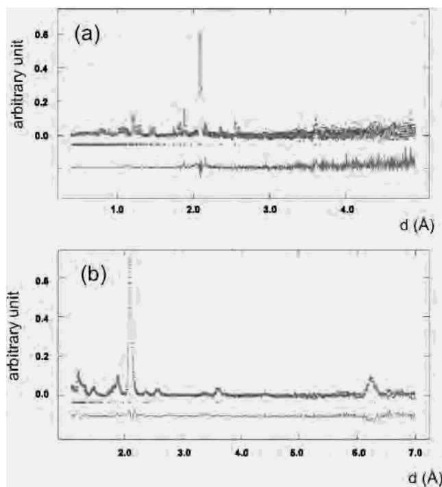
Figure 3. Time of flight (TOF) neutron powder diffraction patterns observed and calculated of \zeta_2 -GaFe. The measurement have be carried out at \theta = 3.2^\circ . The Rietveld refinement of neutron powder diffraction data for GaFe. Part a represents 1 of the 8 individual histogram of the 140^\circ detector banks and part b represents 1 of the 12 individual histogram of the 40^\circ detector banks. The upper curve is the experimental data, and the lower is (experiment-calculated) on the same scale.
