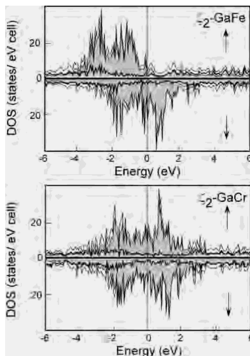
Figure 8. Total density of states (TDOS) and different partial densities of states (PDOS) for the spin-polarized calculations on \zeta_2 -GaM (M = Cr and Fe).
